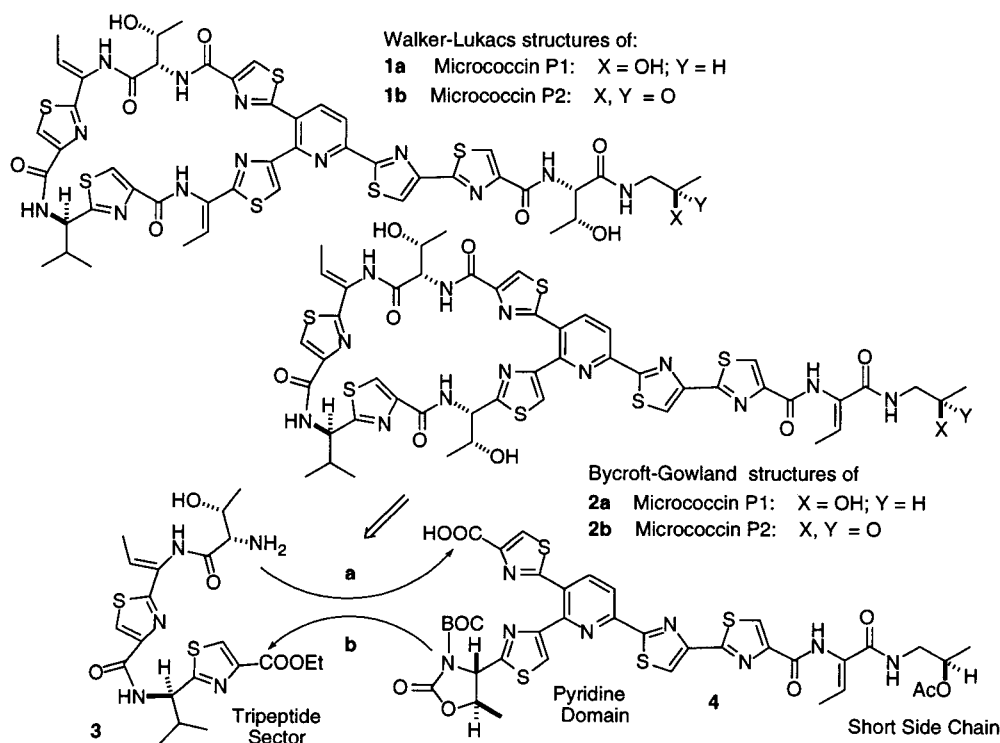
Figure 1. Proposed structures of micrococcin P1 and P2 and retrosynthetic dissection thereof.
